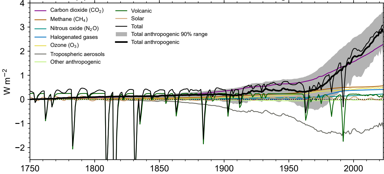
(b) Time evolution of effective radiative forcing 1750-2023
