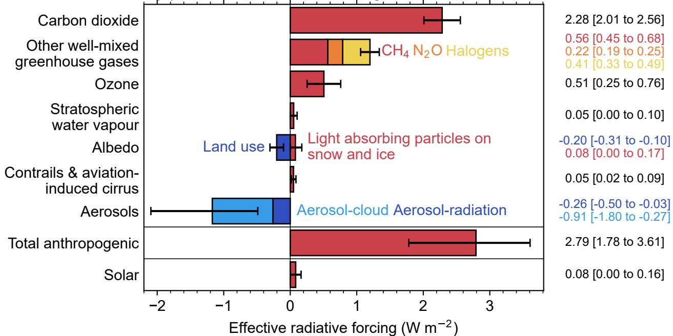
(a) Effective radiative forcing from 1750 to 2023
